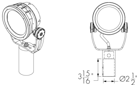
TN2 - Tenon adapter to fit on 2 3/8 in O.D. tenon Vertical mounting only. Consult factory for horizontal mounting.
